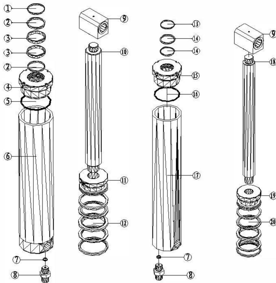
Hydraulic cylinder exploded schematic
